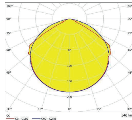
Photométrie AP5-LED CGS comp./PLC
